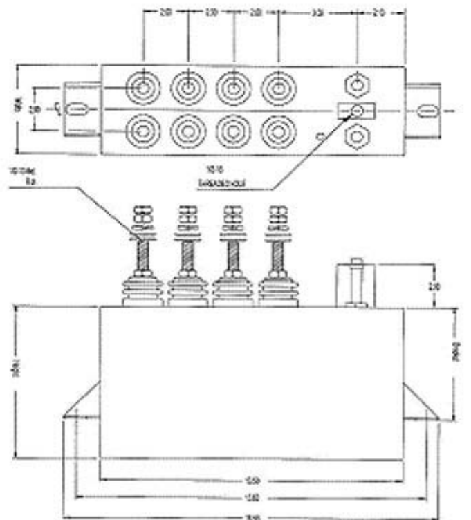
Typical AR Series Can Configurations
